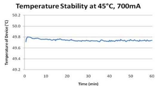
FIGURE 1: The one hour temperature stability of the device, being driven at 700mA, when the case temperature is set to 45°C.
