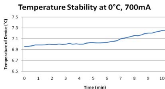
FIGURE 3: The ten minute temperature stability of the device, being driven at 700mA, when the case temperature is set to 0°C.
