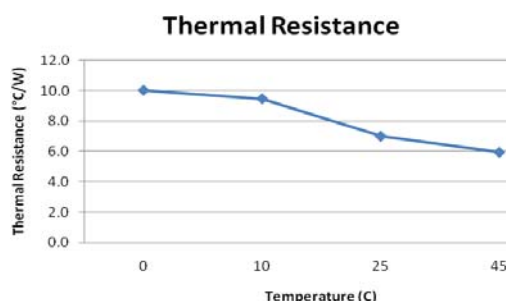
FIGURE 4: The thermal resistance as a function of the temperature.
