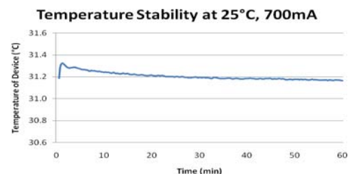
FIGURE 2: The one hour temperature stability of the device, being driven at 700mA, when the case temperature is set to 25°C.
